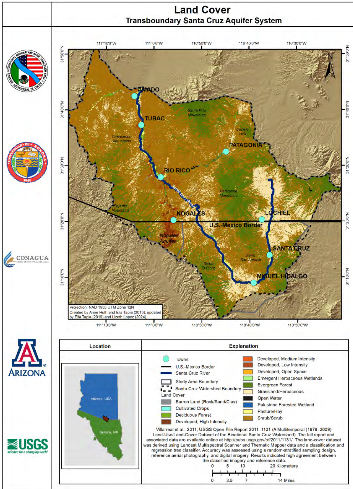
Figure 2.4 Derived land cover in the Transboundary Santa Cruz Aquifer System (modified from Villarreal et al., 2011).
