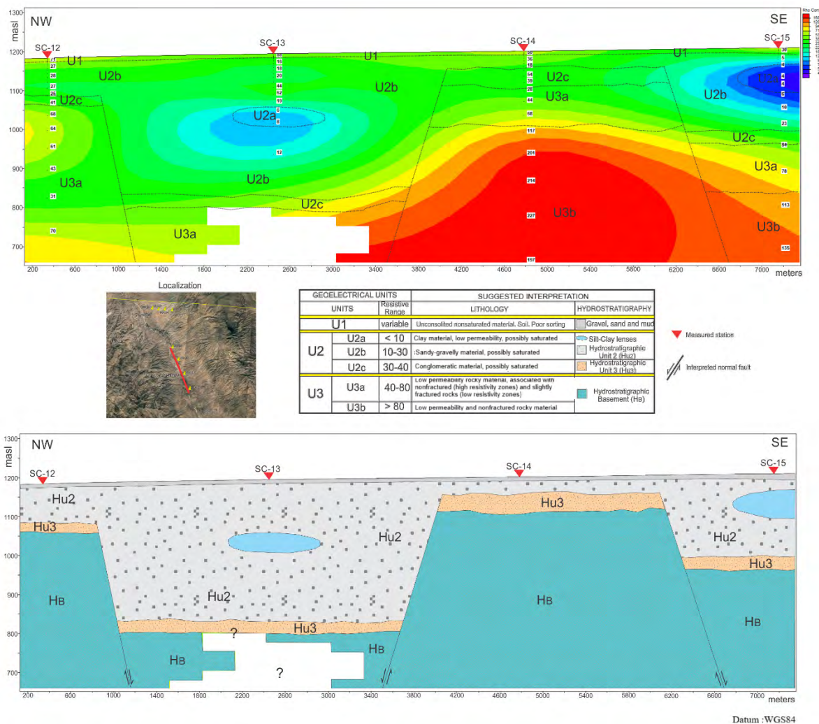
Figure 5.3 Interpreted hydrostratigraphic profile (bottom) from the resistivity profile (top) from the southwestern edge of the Sierra San Antonio on the Mexican side of the TSCAS (this was interpreted based on the data in Figure 4.7).
